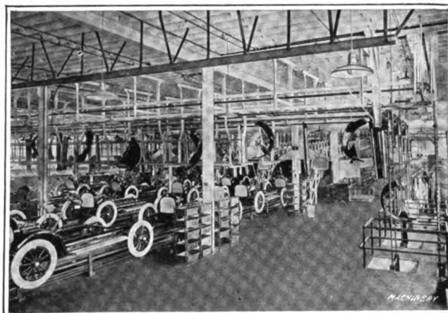
Fig. 38—In handling the progressive assembly of automobiles, the Willys-Overland Co. has tracks down which the cars are run during the process of assembly. Overhead trolley systems running at right angles to the line of travel of assembling tracks carry various parts to the assemblers
